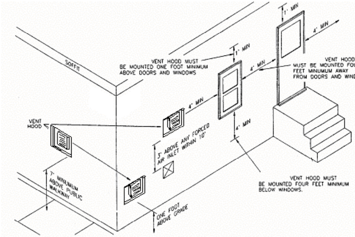
Installation vent terminator Clearance
